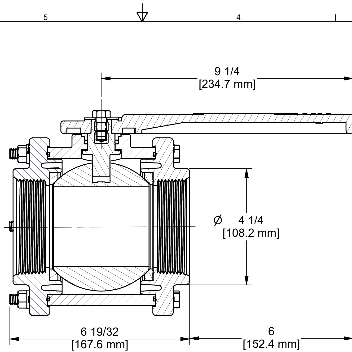
SECTION A-A SCALE 3/5
